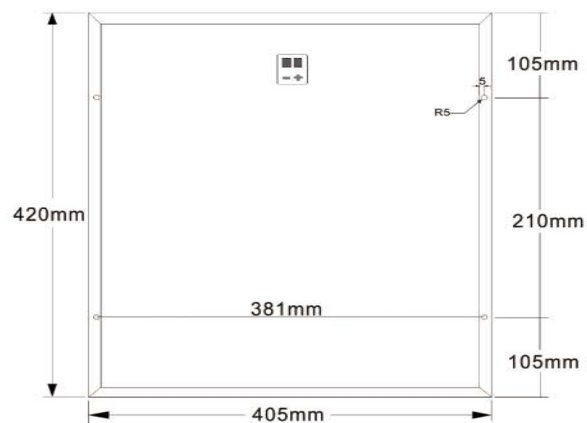
Mechanical Diagrams
